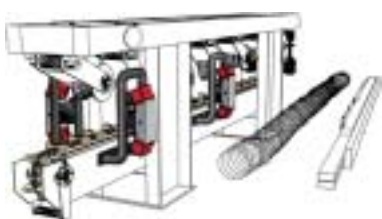
Illustration of in-line scanners (red) imaging a log and modeling board output.
